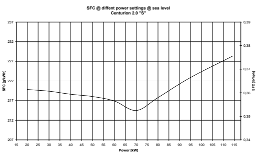
SFC at different power settings at sea level
