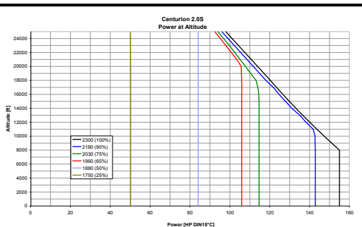
Power at altitude
